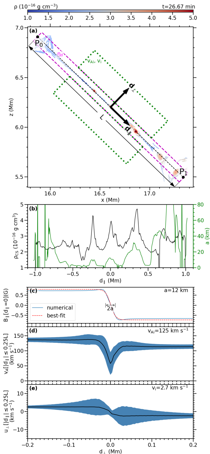
Fig. 4: Characteristics of the current sheet (case 8kU6). Panel (a): Mass density \rho in the current sheet, mapped for L_B \leq 20 km. The dashed line with endpoints P_0 to P_1 marks the current sheet, with coordinate axes for d_{||} and d_{\perp} plotted in. Diffusion and inflow regions are delimited by magenta and green rectangles, respectively. Panel (b): Average density \rho_{CS} (black curve) and width a (green curve) of the current sheet. Panel (c): Parallel component of magnetic field, B_{||} (blue), across the current sheet and the best-fit (red) curve used to estimate a at d_{||} = 0 . Panels (d) and (e): Alfvén velocity v_A (d) and perpendicular velocity u_{\perp} (e) across the current sheet. Blue area maps the ranges of all values for |d_{||}| \leq 0.25L , and black curve plots the average. Estimated inflow region mean values are printed in top right corner.
