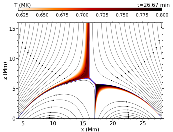
Fig. 2: Temperature and magnetic field topology taken from simulation case 8kU6. A movie of the time evolution of the map for t \in [0, 40] min is available online.
